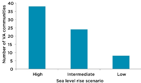
FIGURE 2. Number of Chronically-Inundated Communities In Virginia In 2100 Under Three Scenarios.
