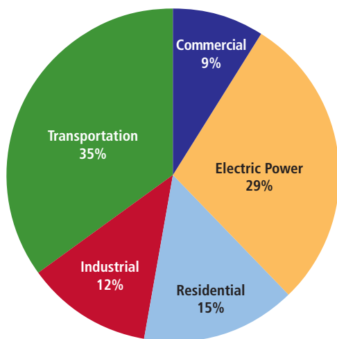
FIGURE 1: Northeast States—Regional Emissions of CO 2 by Sector, 2003
