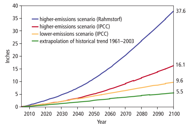
FIGURE 4: Projected Rise in Global Sea Level Relative to 2005
